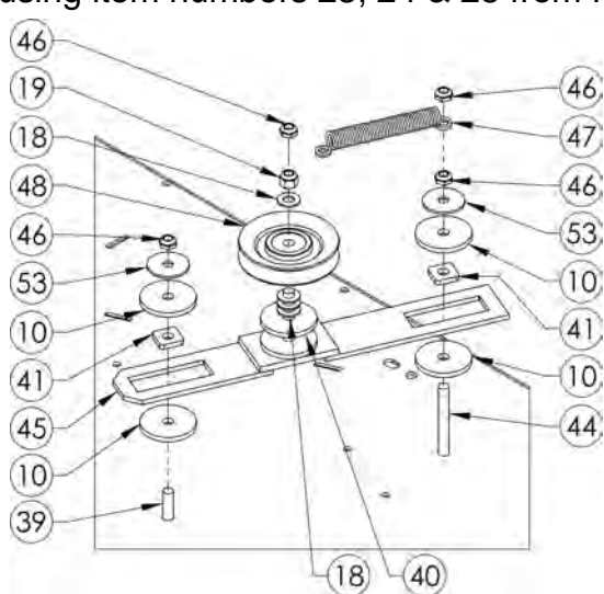
INSIDE IDLER DETAIL
