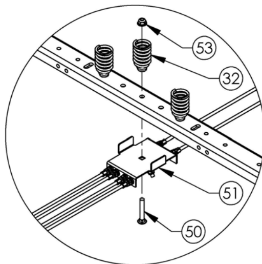
BRAKE & HYDRO BYPASS ASSEMBLY
